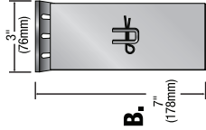
B. ELECTRO/1 EXTENDED DRIVE-END BRACKET
