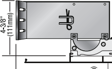
E. ELECTRO/3 DRIVE-END BRACKET
