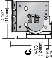
C. ELECTRO/2 DRIVE-END BRACKET
